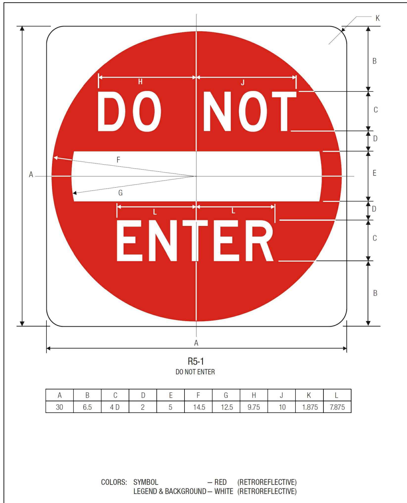
R5-1 'DO NOT ENTER' SIGN
